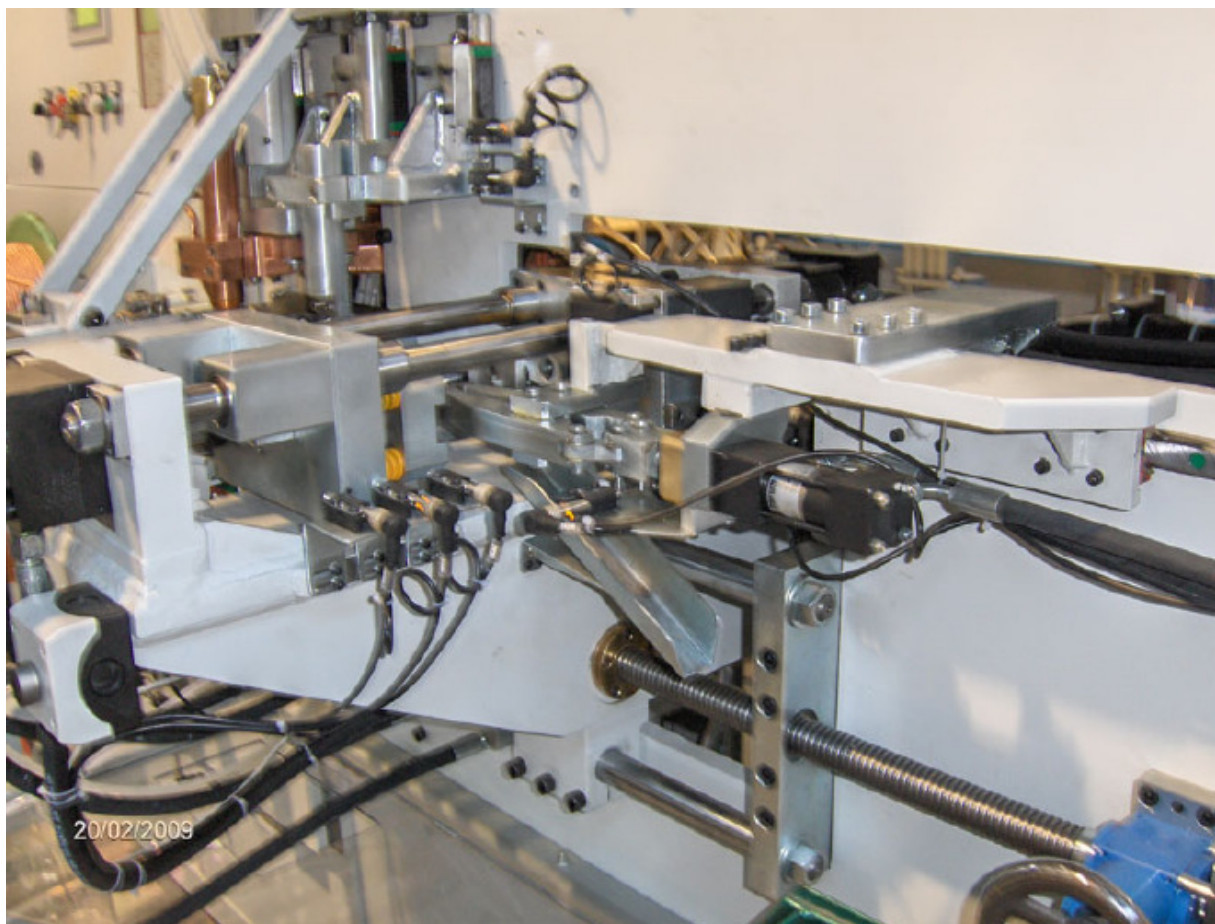
VIEW OF THE HAULAGE AND CUTTING SYSTEM.
