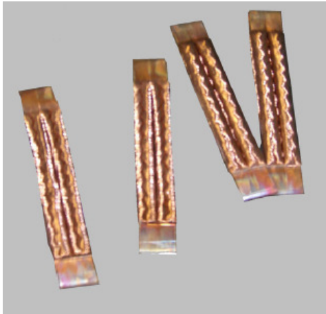
EXAMPLE OF PROCESSED STRANDED WIRES (45 sq. mm.)
